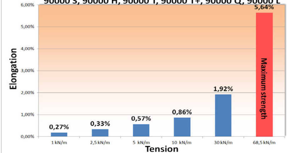
Elongation at specific tension
