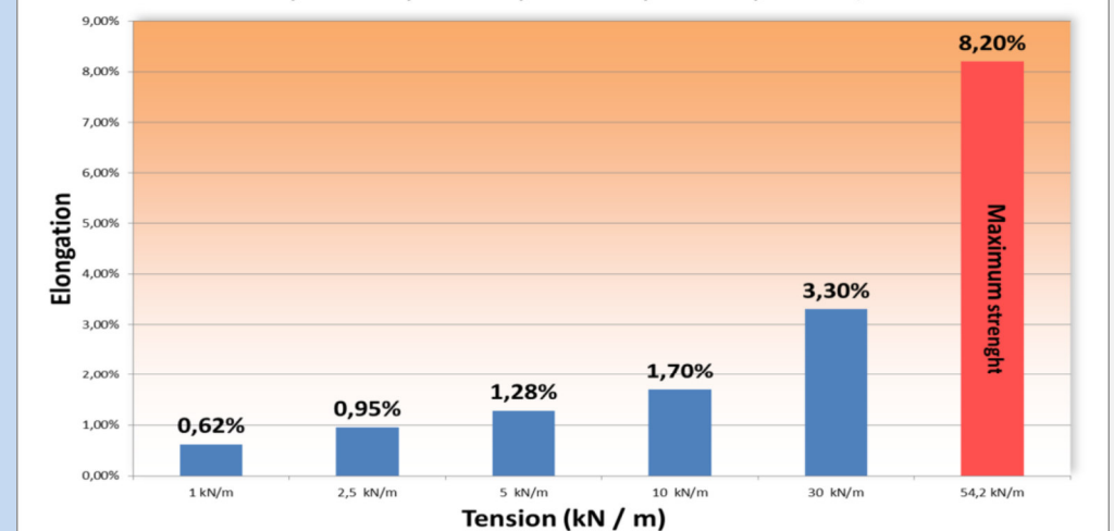
Elongation at specific tension 60000 SL, 60000 HL, 60000 TL, 60000 TL+, 60000 LL, 60000 QL
