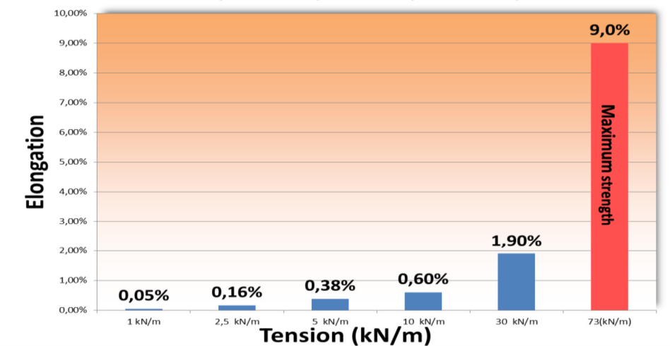
Elongation at specific tension 70000 S7L, 70000 H7L, 70000 T7L, 70000 T7L+, 70000 Q7L
