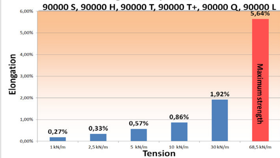
Elongation at specific tension
