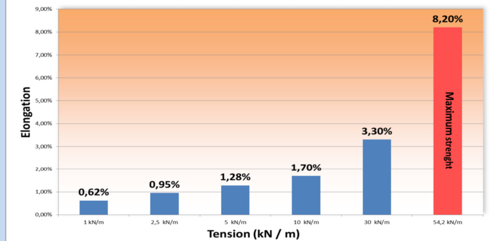
Elongation at specific tension 60000 SL, 60000 HL, 60000 TL, 60000 TL+, 60000 LL, 60000 QL
