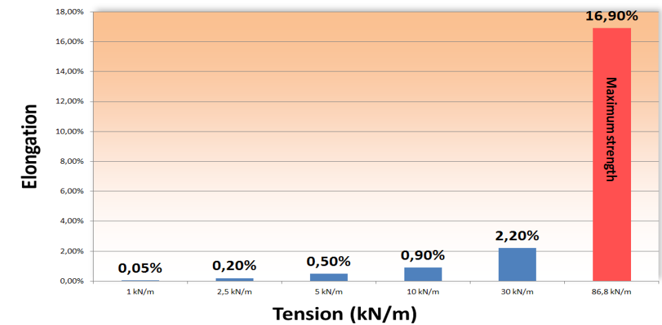
Elongation at specific tension 70000 S7, 70000 H7, 70000 T7, 770000 S7-A, 70000 L7, 70000 Q7
