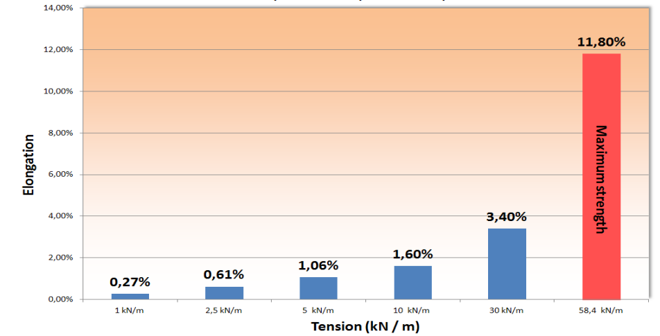
Elongation at specific tension 43000 FSL, 43000 FHL, 43000 FTL, 43000 FLL
