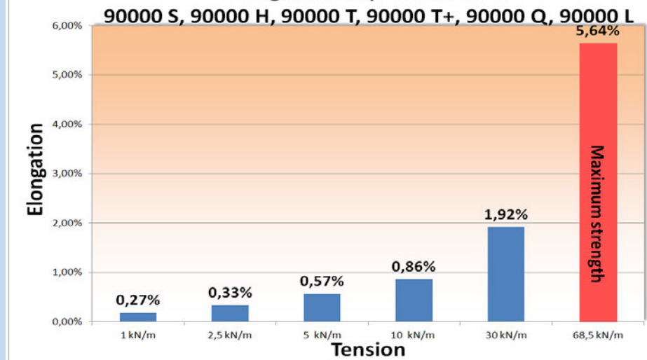
Elongation at specific tension
