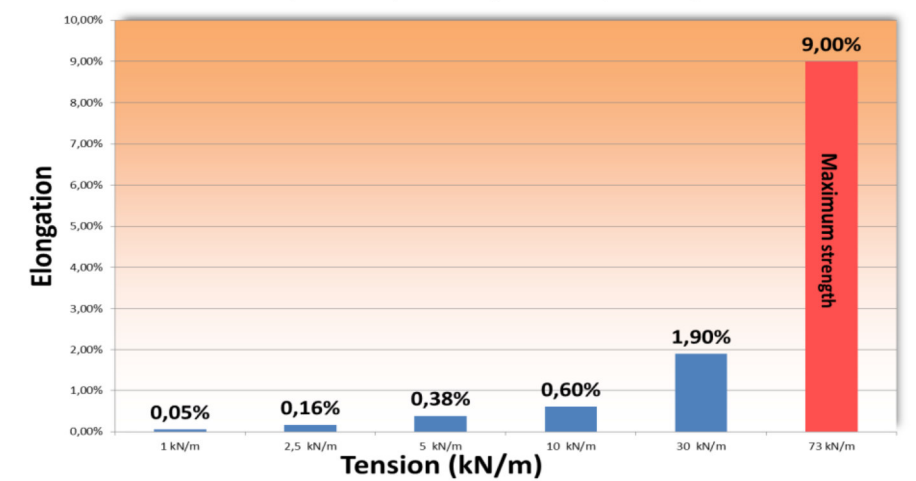
Elongation at specific tension 70000 SL, 70000 HL, 70000 TL, 70000 TL+, 70000 QL
